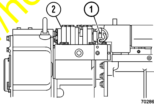
Figure 3. Installation of Mounting Elbow
