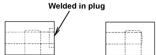
Modified design eliminating the welded in plug
