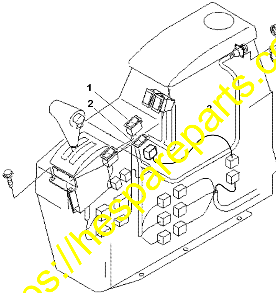
CONSOLE BOX
