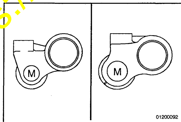
Figure 1 New Valve Camfollower (left), New Injector Camfollower (right)
