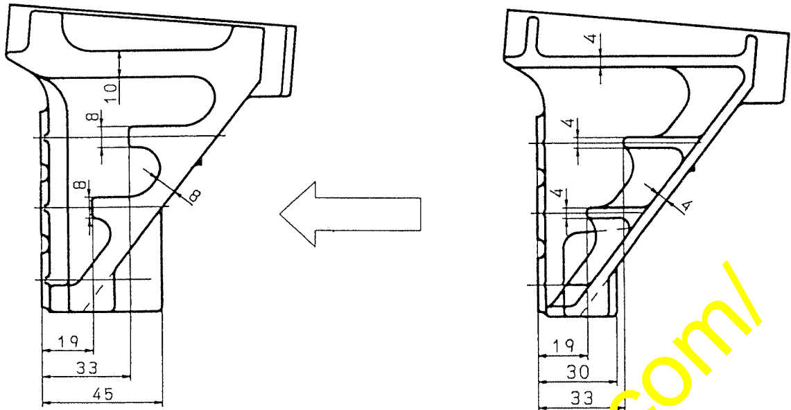
Reinforced bracket 6152-25-6111
